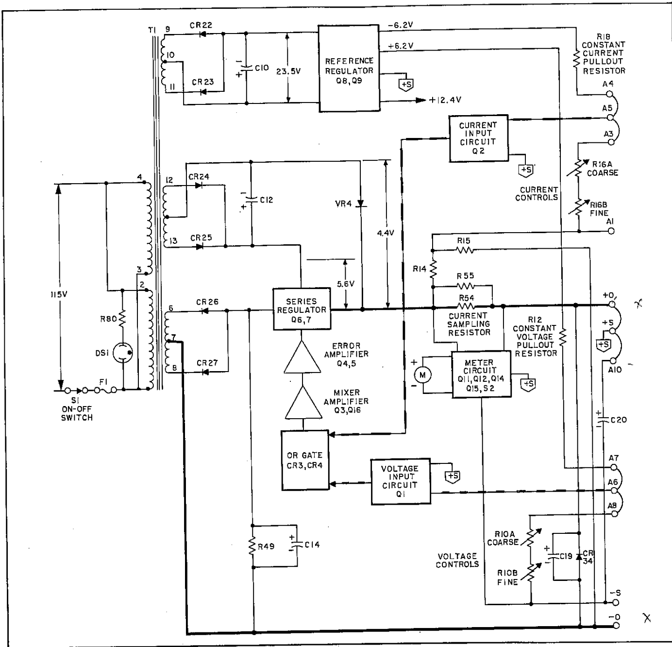
Figure 4-2. Simplified Schematic
